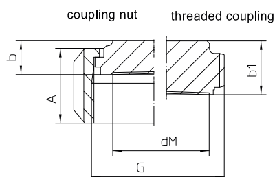
Sanitary pipe connection per IDF (BS 4825-4) for pipes per BS 4825-1
