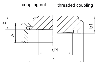
Sanitary pipe connection per SMS 1145 for pipes per ISO 2037
