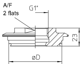
VARIVENT® connection for VARINLINE® access unit
