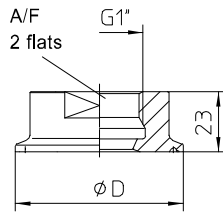
clamp-connection
