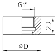
welded socket (welded in accordance with operating instruction)
