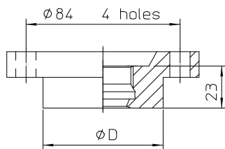
DRD-connection
