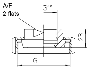
tapered coupling with union nut DIN 11851
